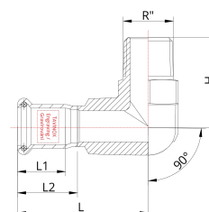
Technical drawing
