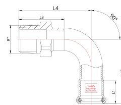
Technical drawing
