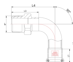
Technical drawing
