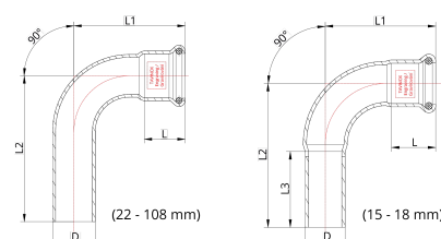
Technical drawing
