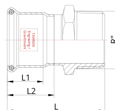
Technical drawing
