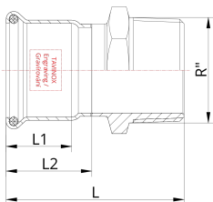
Technical drawing
