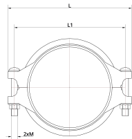
Technical drawing
