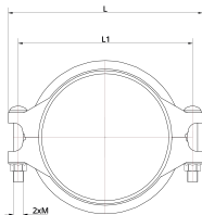
Technical drawing
