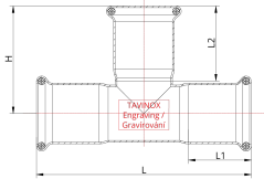
Technical drawing
