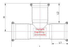
Technical drawing
