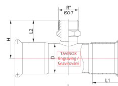
Technical drawing
