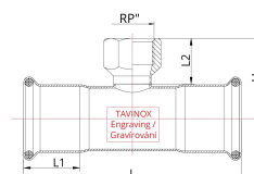
Technical drawing
