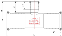
Technical drawing
