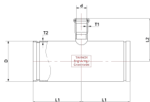
Technical drawing
