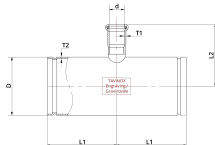
Technical drawing
